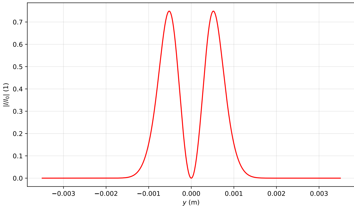
Intensity profile I(x=0, y, z=0.557)/I_0 , P_{in}=1.0P_{cr} , artificial time
